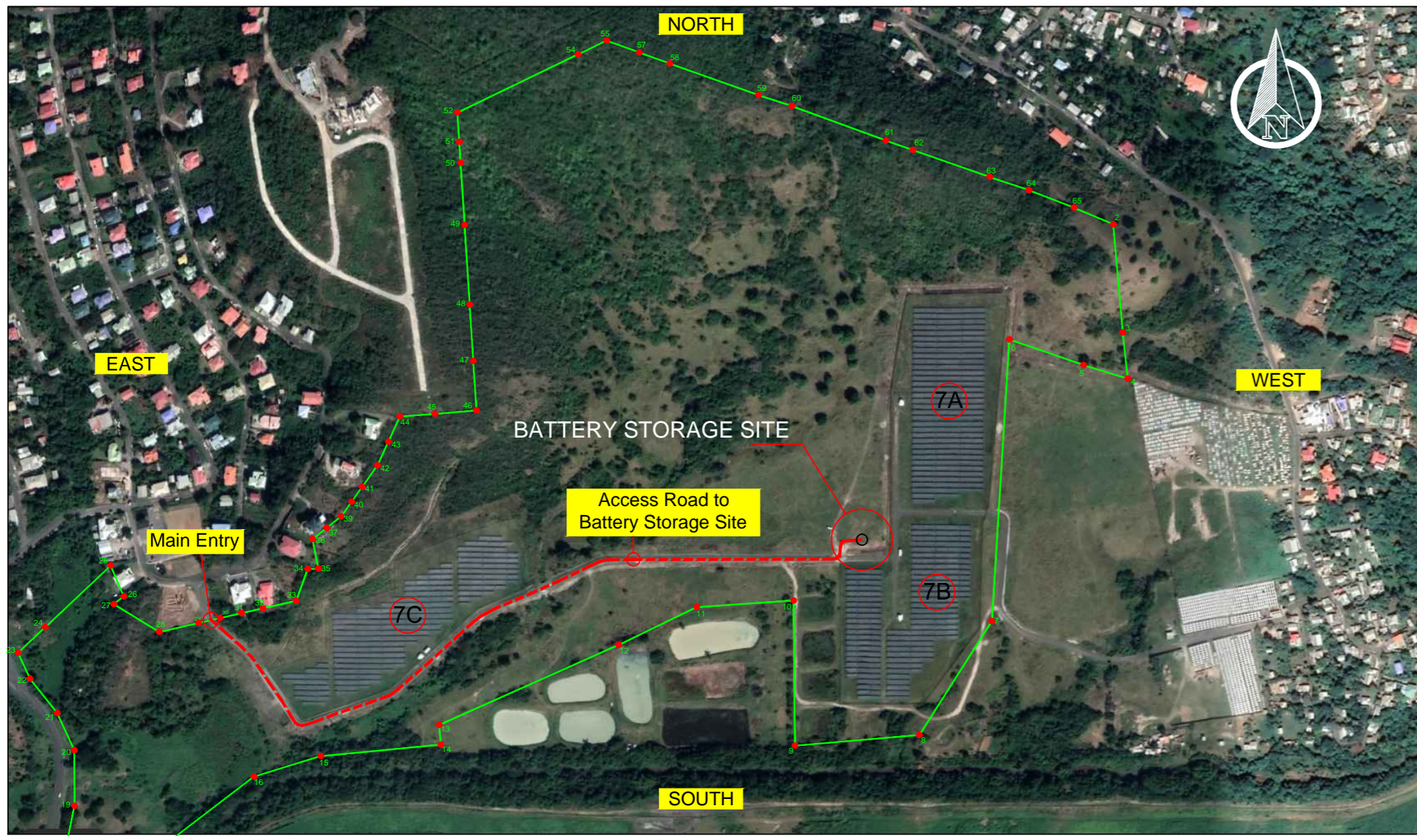
PLAN VIEW OF THE 3MW SOLAR FARM
